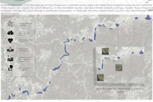
Potential detention basins along the Ahr river
