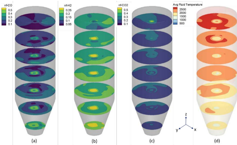
Figure: Entrained gasifier parameters at different levels in the reactor: Instantaneous mole fraction for gas species: - (a) CO, (b) H 2 , (c) CO 2 and (d) time average fluid temperature
