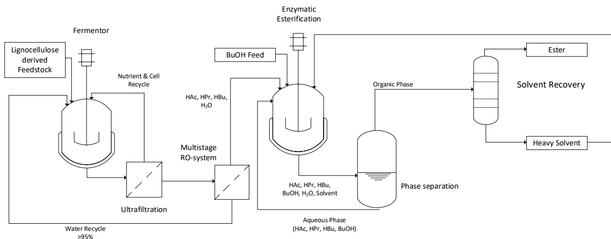
Figure 1: Initial flowsheet and downstream processing
