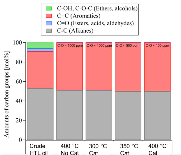
Figure 2: Product fractions from catalytic and non-catalytic HDO of HTL crude.
