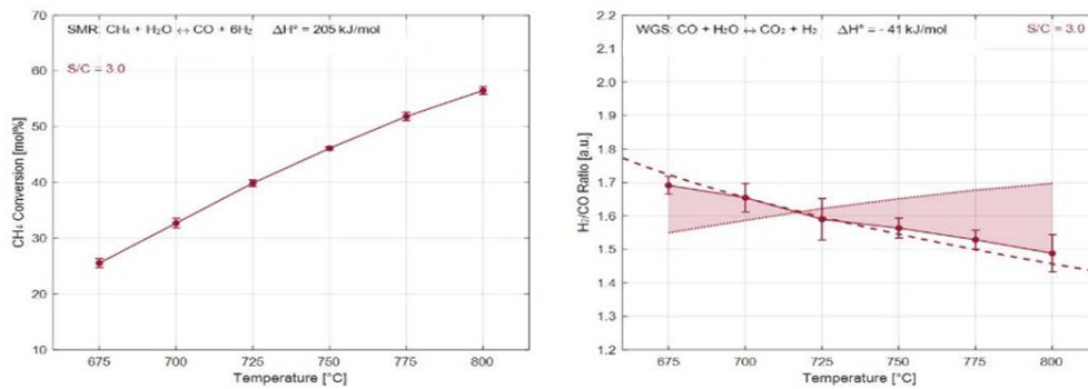
Figure: Example showing the methane conversion (left graph) and resulting H 2 :CO ratio (right curve) as a function of the temperature over a supported Co-Ni catalyst (run at high space velocity to investigate the kinetics of the reaction). Dashed line in the right-side graph represents the calculated H 2 :CO ratio assuming WGS equilibrium. The inlet gas composition is based on a typical exit gas from a gasifier, and the experiment here is run with a steam to carbon ratio of 3.
