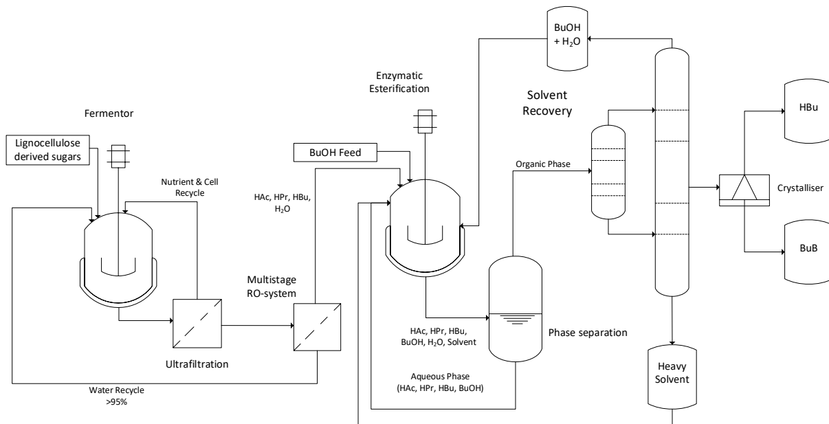
Figure 2: Advanced downstream separation with a multieffect distillation
