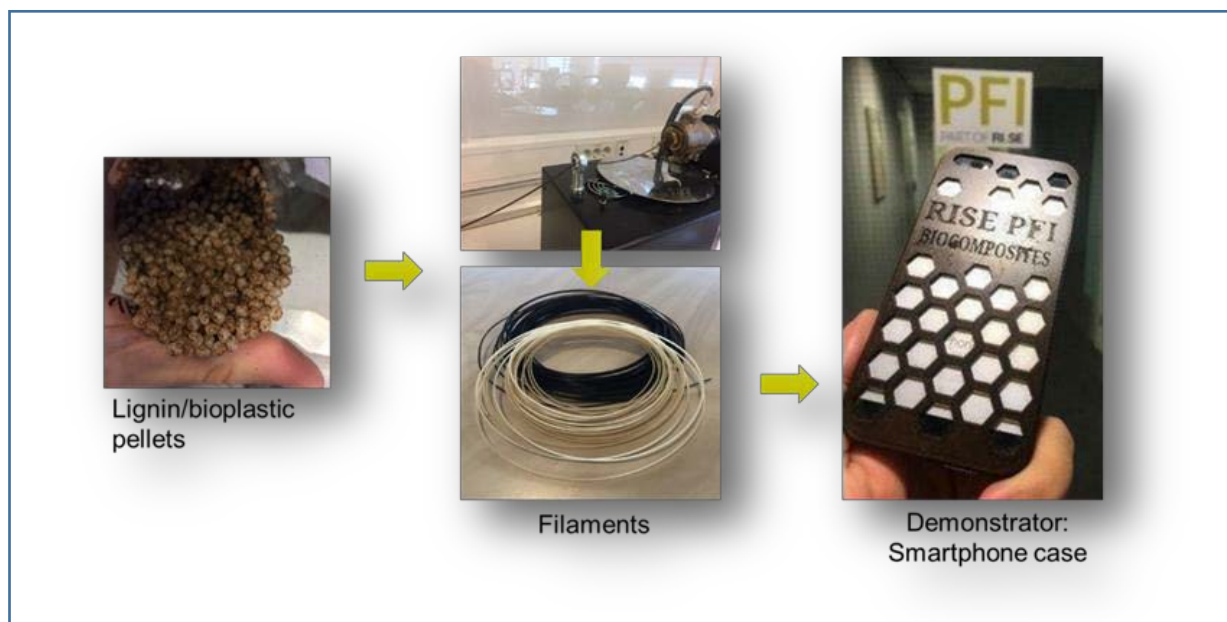
Figure 1: Left) PLA/lignin pellets. Middle) Extrusion of PLA/lignin filament. Right) 3D printed demonstrator of PLA/lignin biocomposites.
